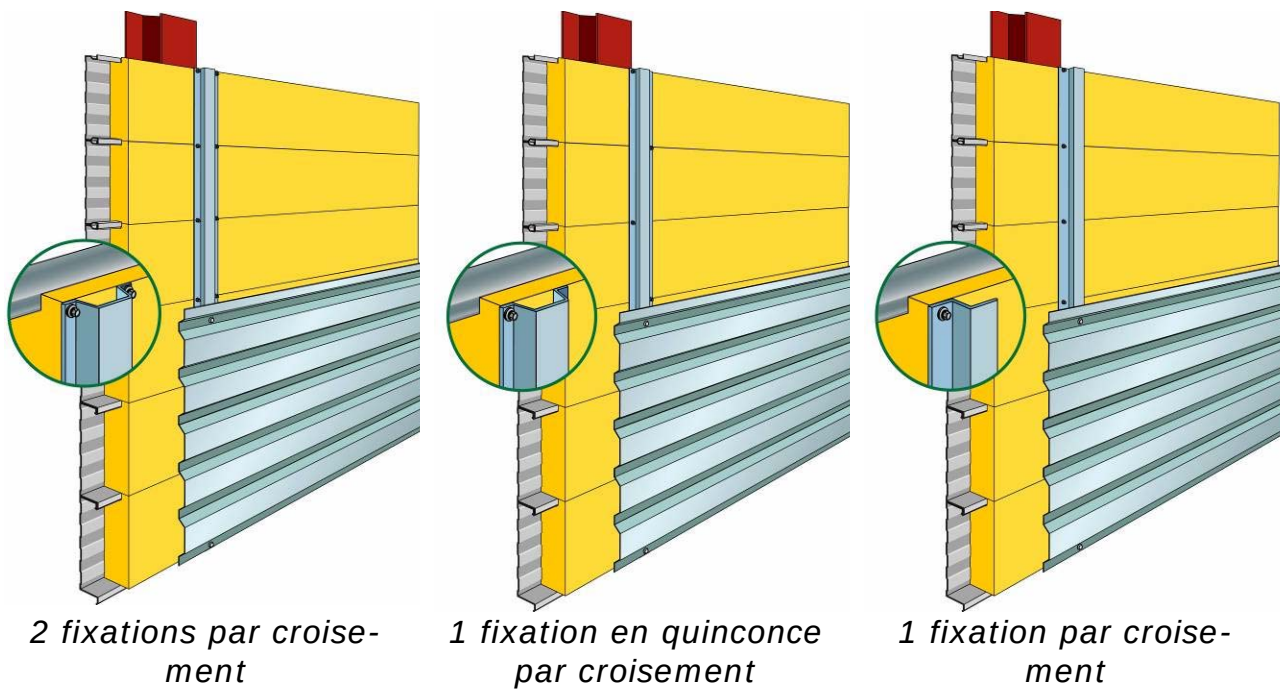
Figure 2 - Bardage Horizontal
