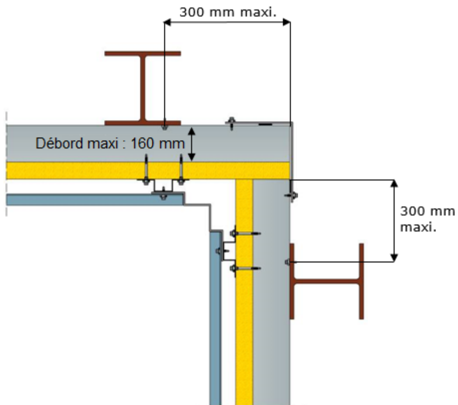
Figure 24 - Angle rentrant
