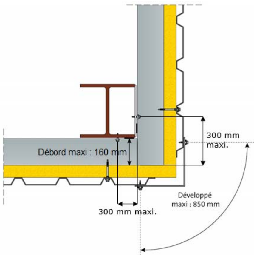
Figure 23 - Angle sortant
