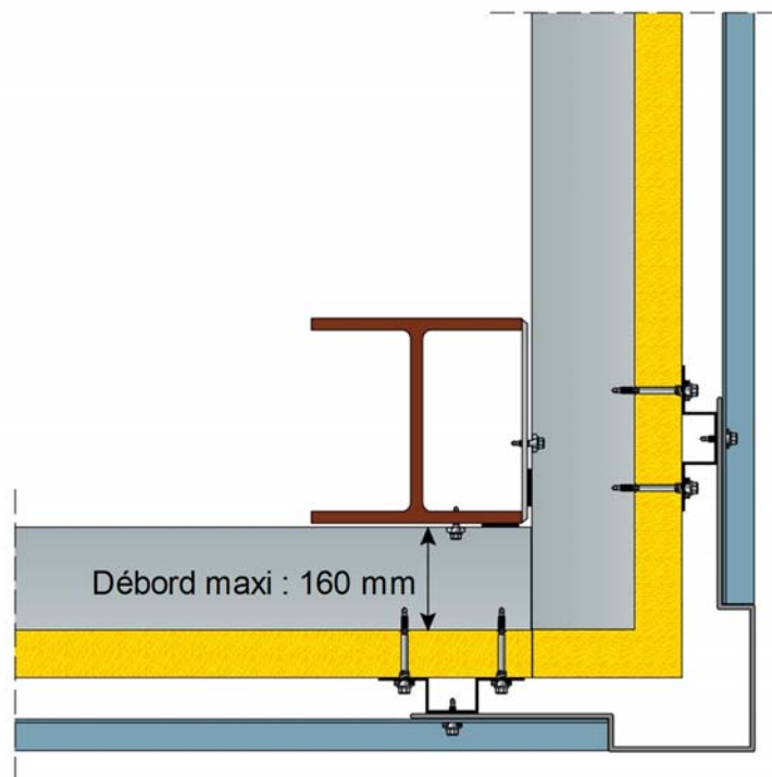
Figure 22 - Angle sortant
