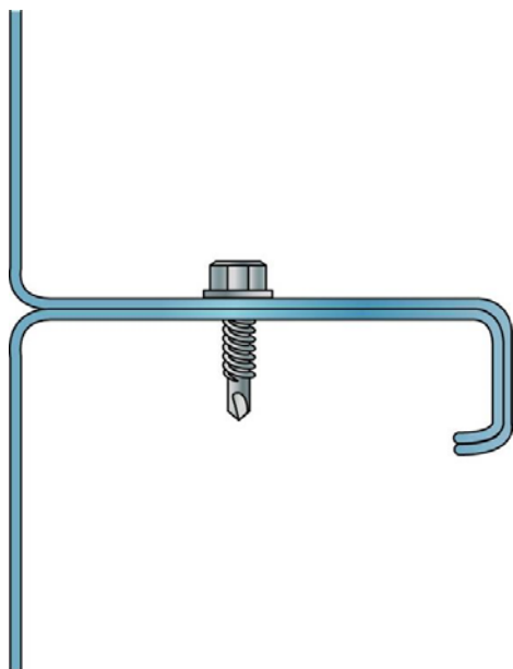
Figure 13 - Couturage inter-plateaux
