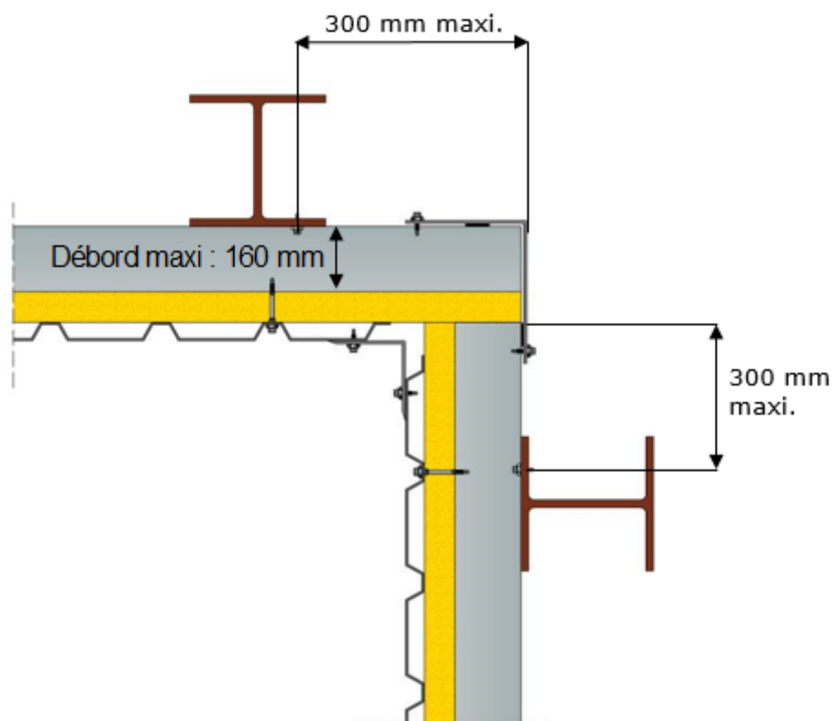
Figure 25 - Angle rentrant
