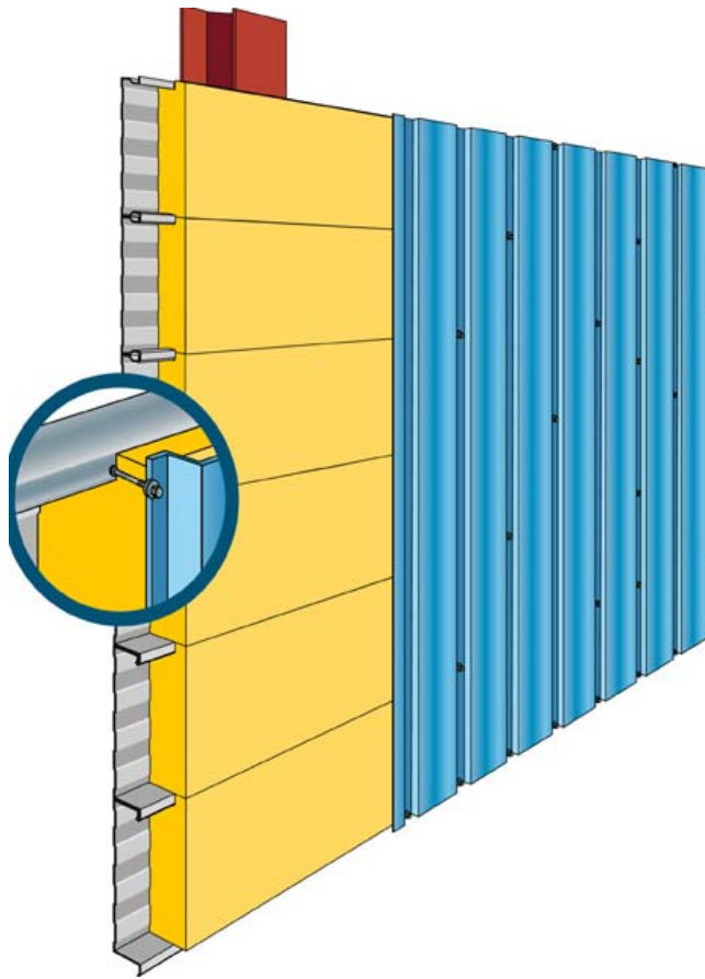
Figure 1 - Bardage vertical
